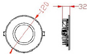
LR-TSLM-126 Weight: 0.5kg
